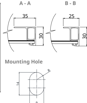
Frame Cross Section
